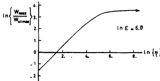
Fig. 6. Plot of \ln \left\{ \frac{W_{max}}{W_{stmax}} \right\} vs \ln(\eta) for the elliptical plate.
